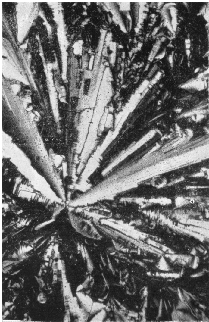
FIGURE 3 Broken-fan texture of the mesophase. Crossed polarizers, \times 500 .
