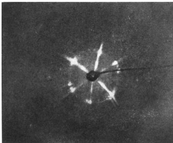
FIGURE 5 X-ray diffraction photograph of a nearly moniodomain specimen of the mesophase of BHp-hexanoate. Specimen to film distance 12.5 cm. Incident beam almost exactly along the six-fold axis.
